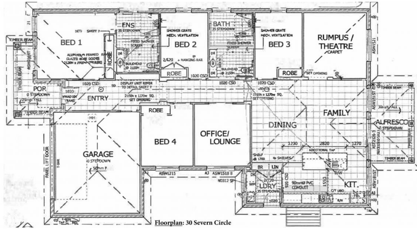
Floorplan: 30 Severn Circle
