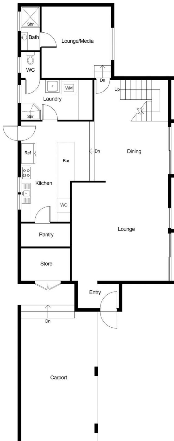
DOWNSTAIRS FLOOR PLAN
