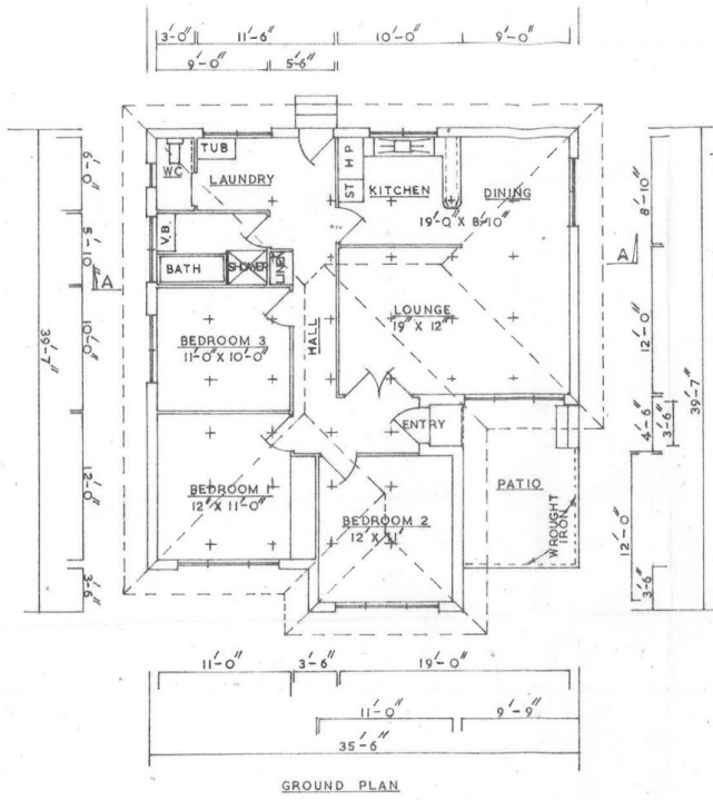
GROUND PLAN
