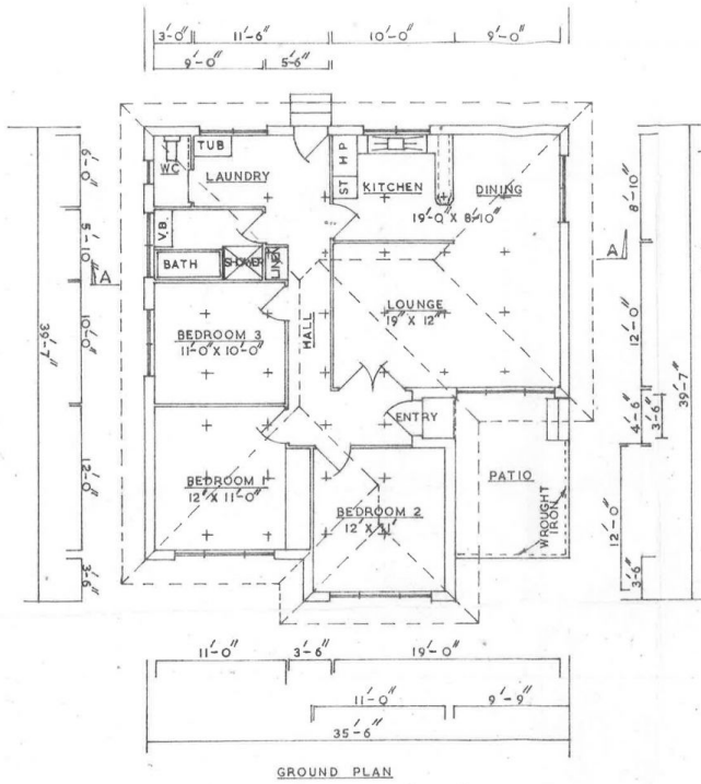
GROUND PLAN
