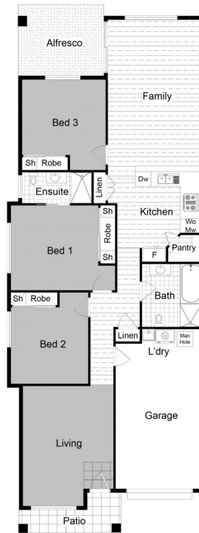
FLOOR PLAN
